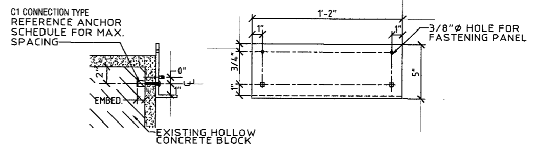
T INTERIOR FASTENING ANGLE ASSEMBLY SCALE: 1-1/2" = 1'-0"
