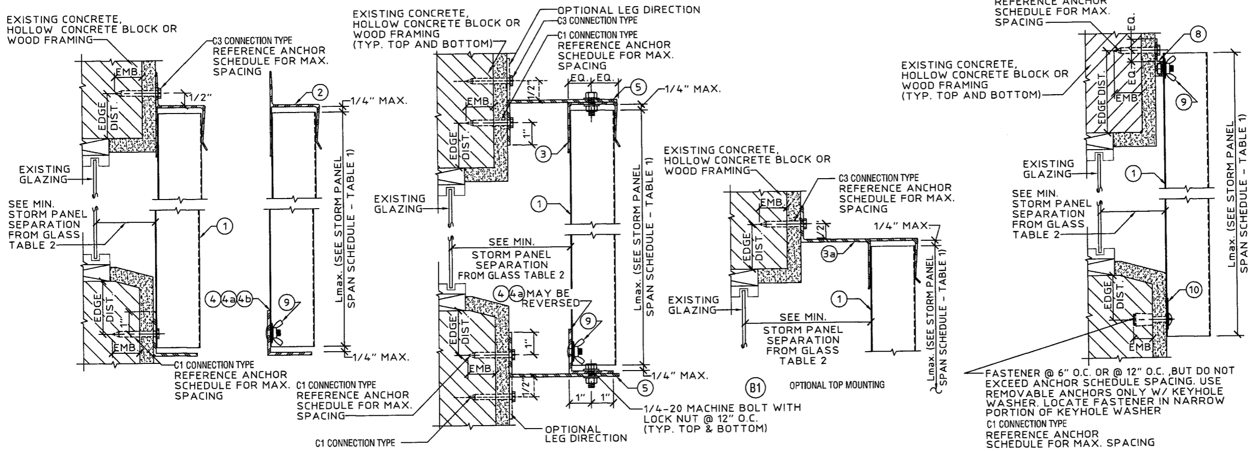
C) "F" TRACK/DIRECT MOUNT SECTION SCALE: 3" = 1' - 0"
