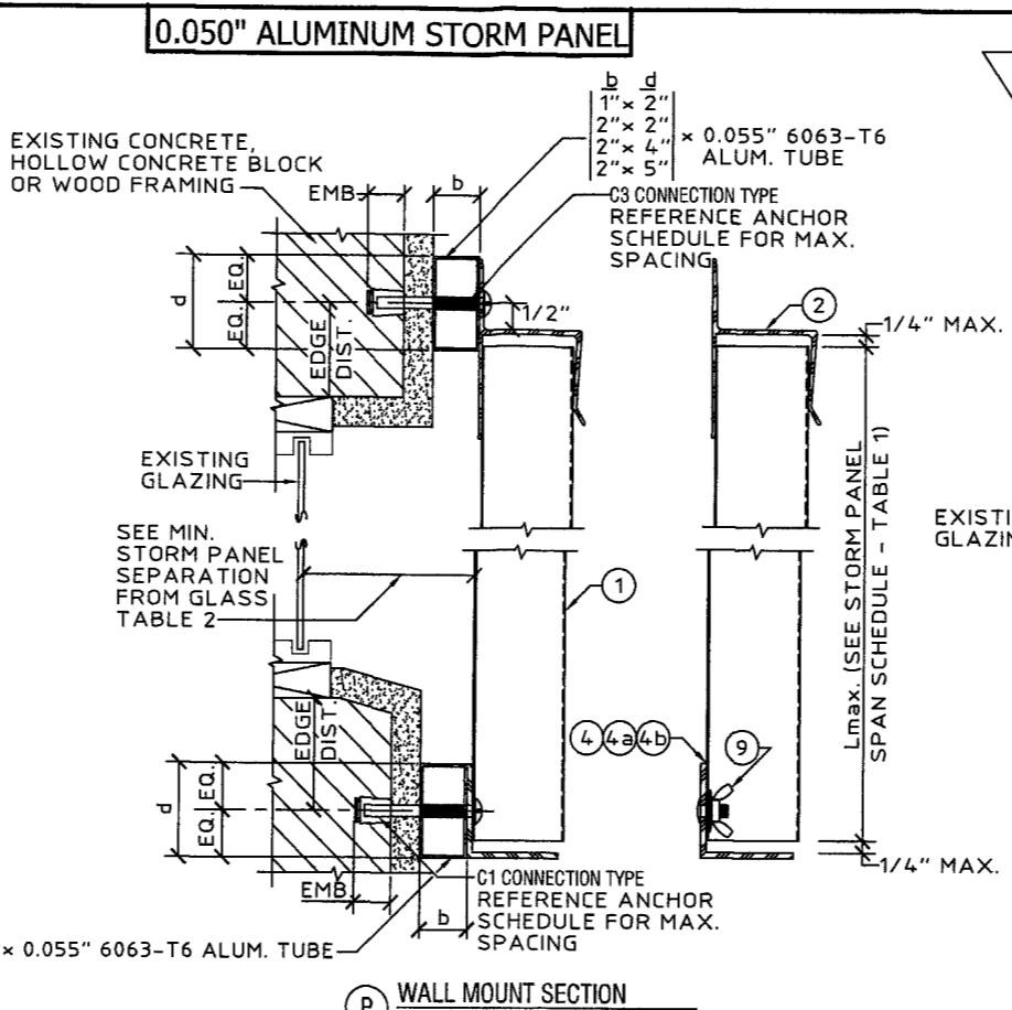
P WALL MOUNT SECTION SCALE: 3" = 1'-0"
